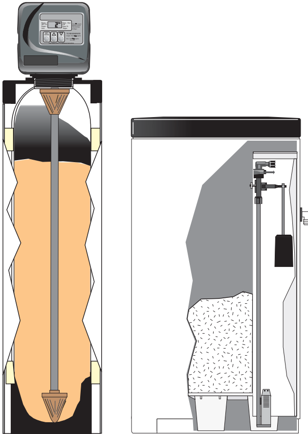
Shown With Optional Thermal Tank Shroud
