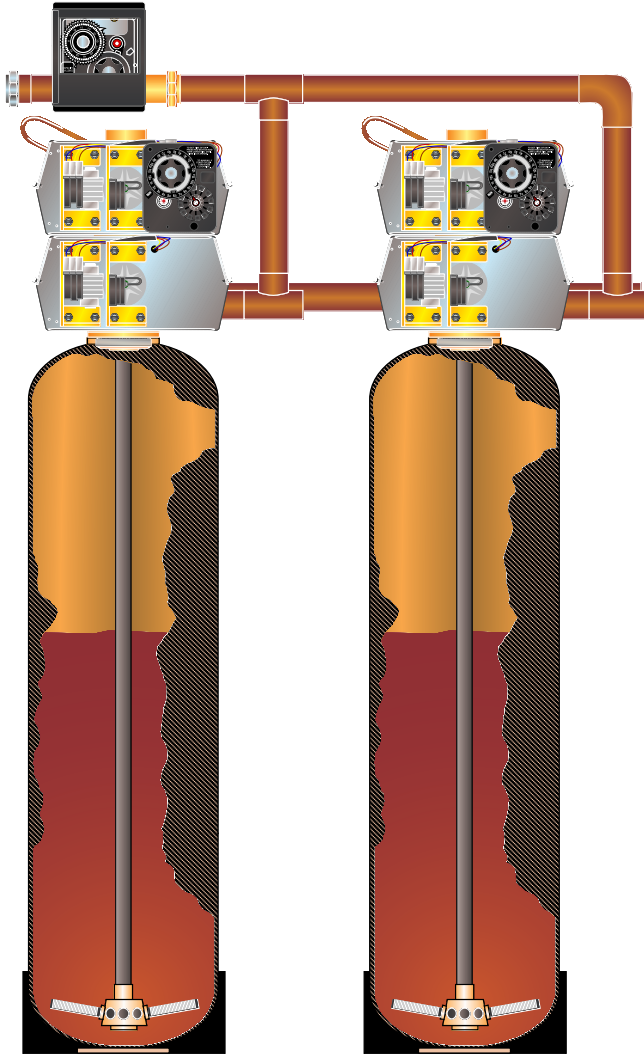
Duplex Configuration (Mechanical Controls Shown)
