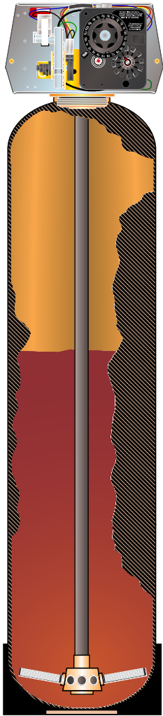
Hub & Lateral Distributor System Shown
