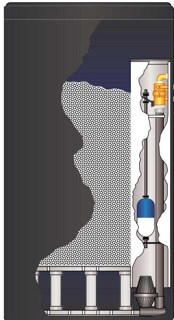
Hub & Lateral Distributor System Shown
